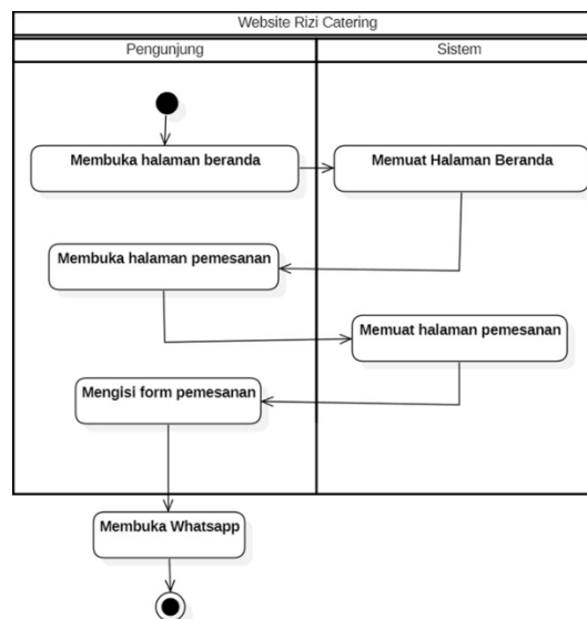
Gambar 2 Activity Diagram
